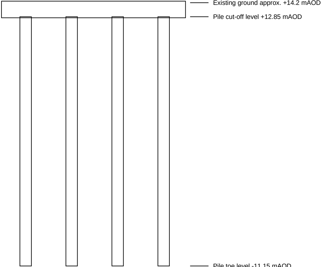
8 No. 900 mm dia. bored piles, 24.0 m long
